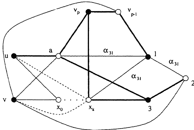
FIG. 10. G_{BAX'}[X] .
